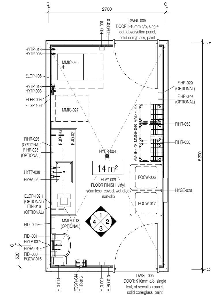
PLAN
