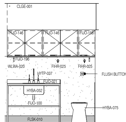
ELEVATION 2 (ALTERNATIVE)
