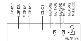
ELEVATION 5 ( 1 : 25 @ A3 )
