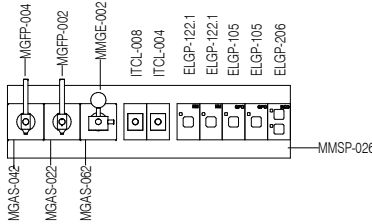
ELEVATION 7 ( 1 : 25 @ A3 )
