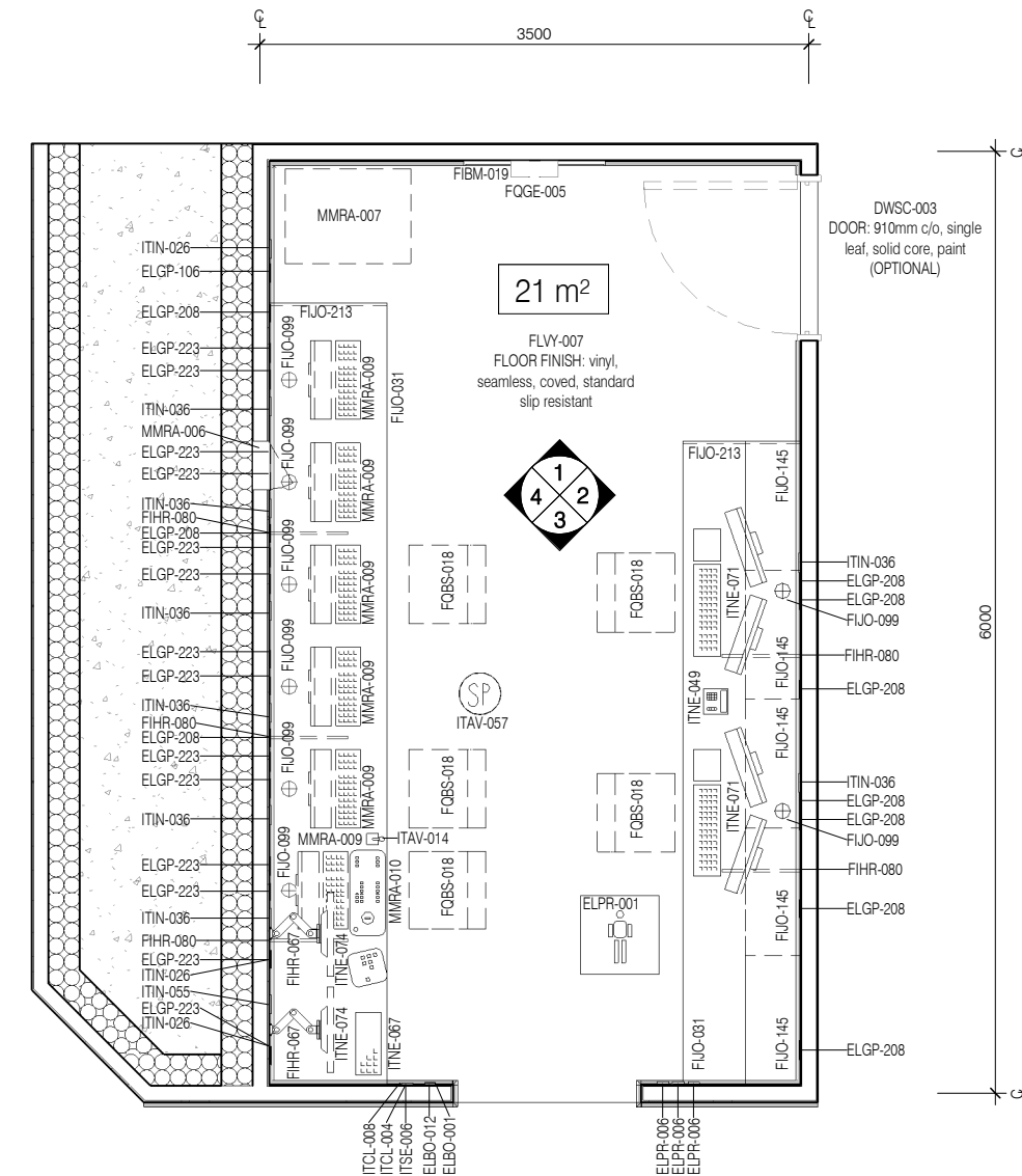
PLAN
