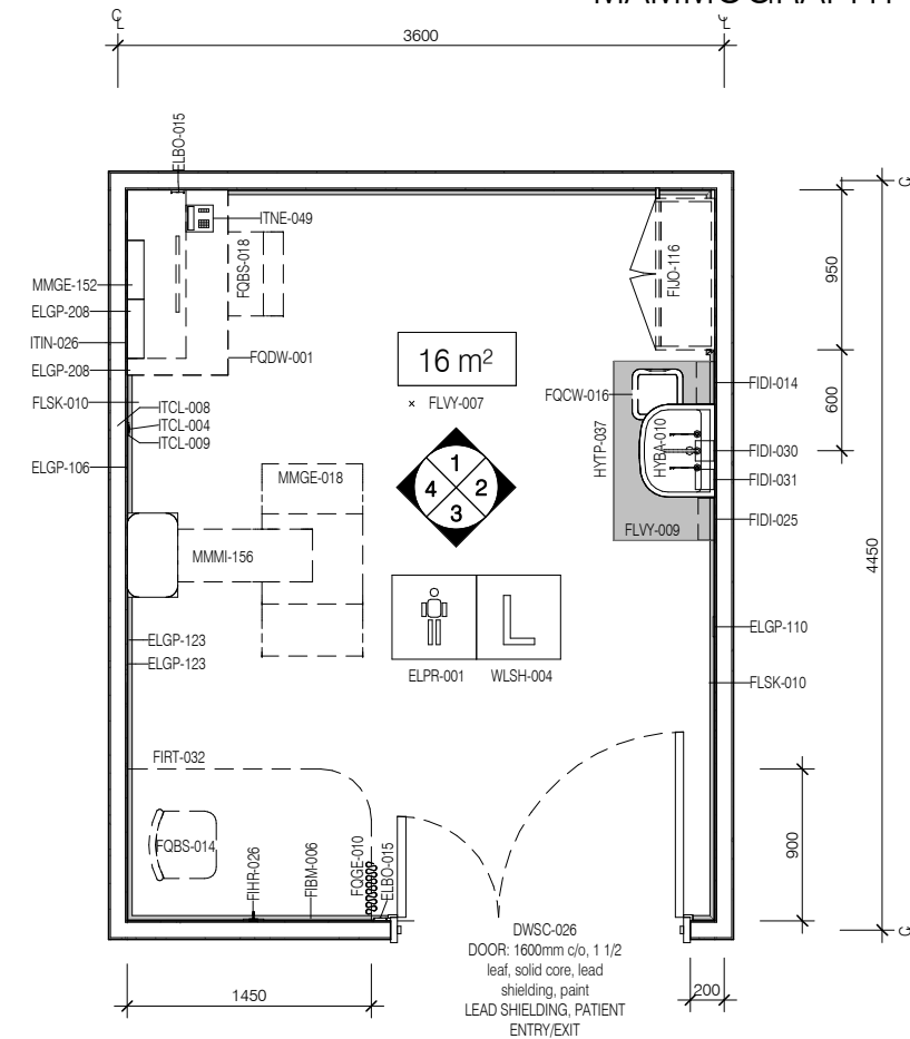
PLAN
