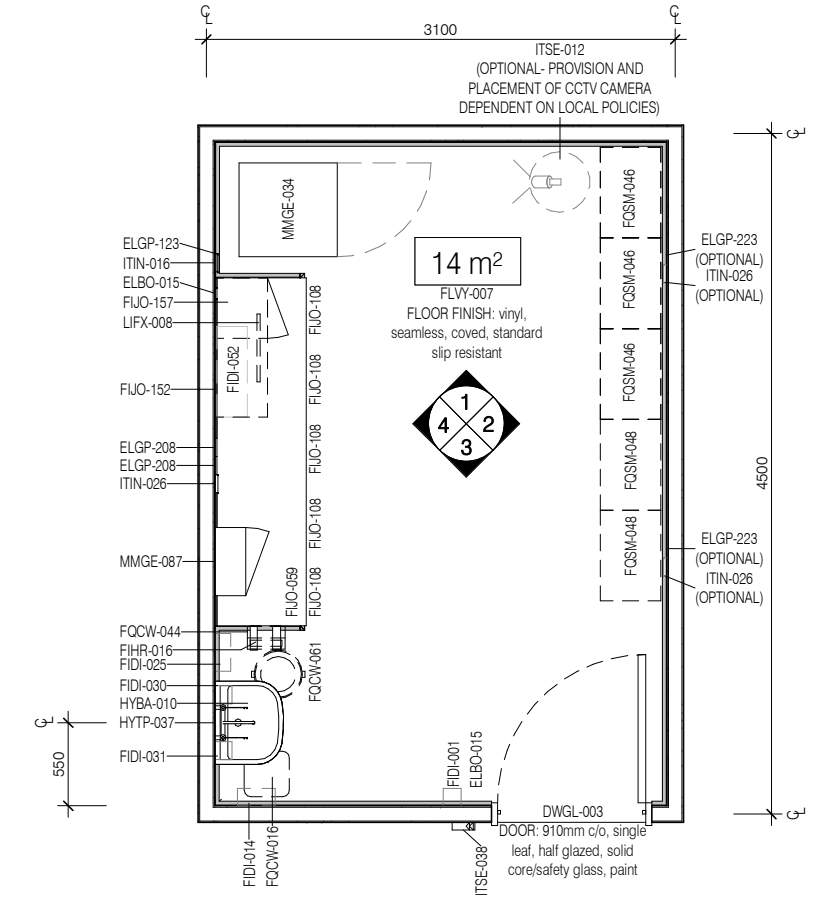
PLAN
