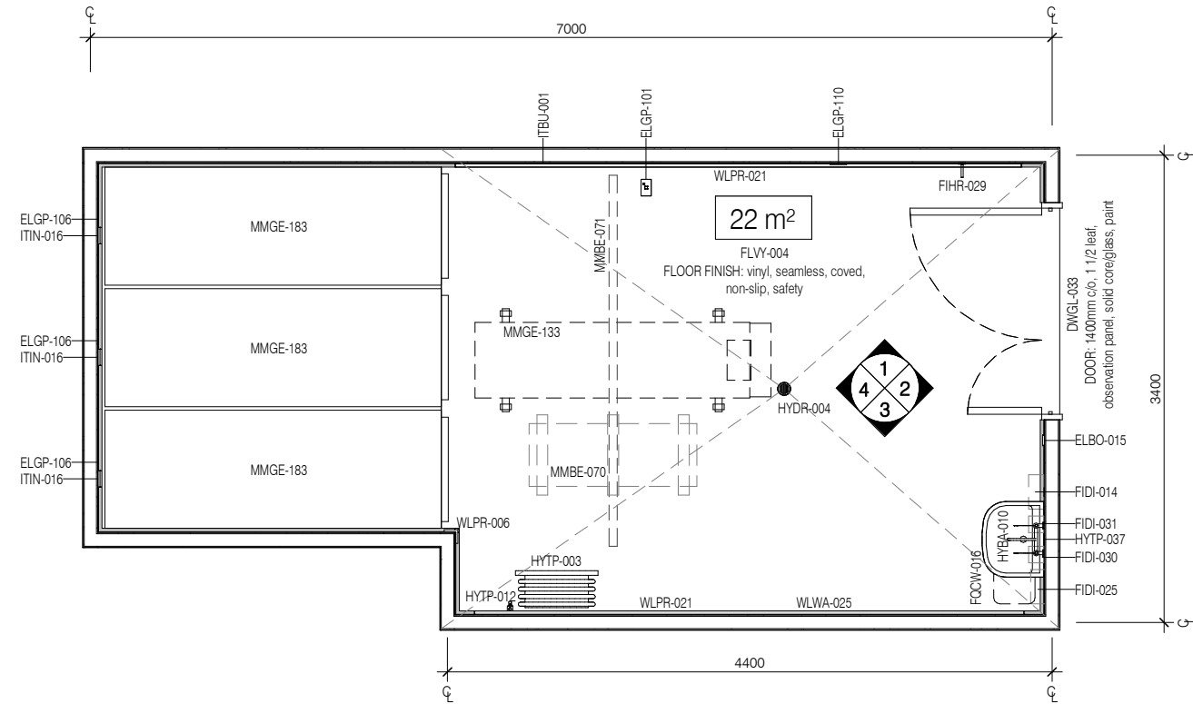
PLAN
