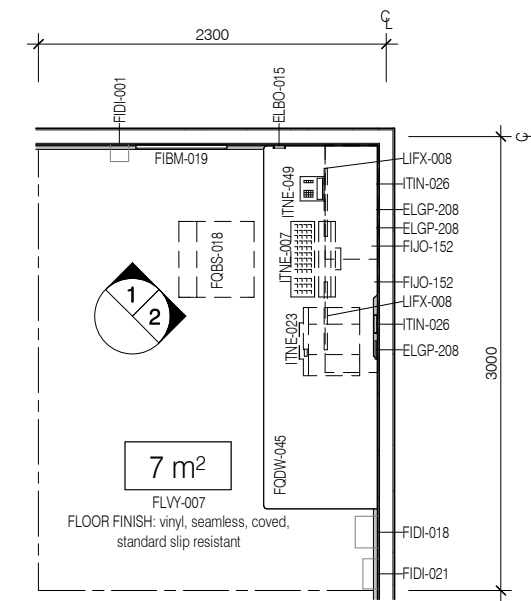
PLAN
