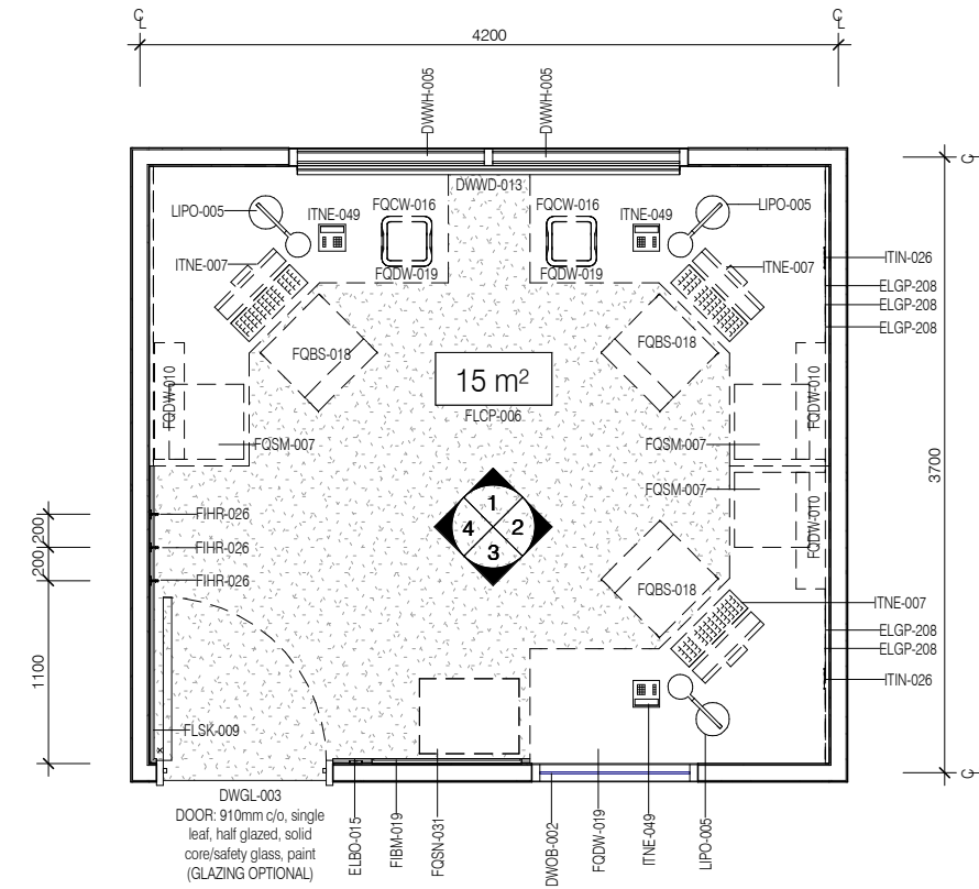
PLAN
