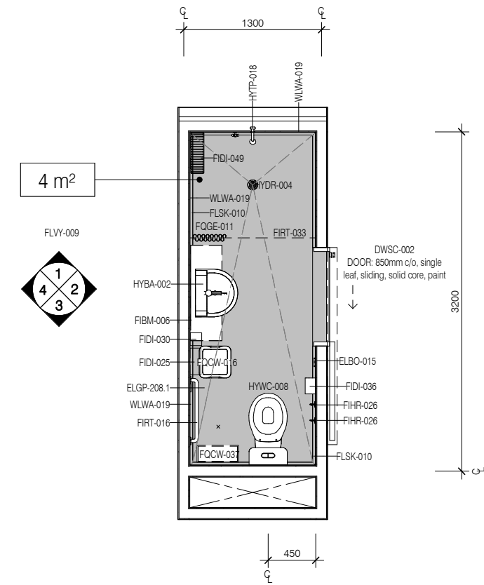
PLAN
