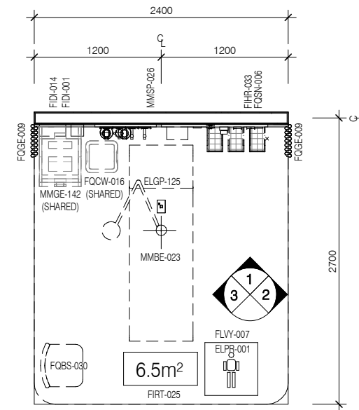
PLAN
