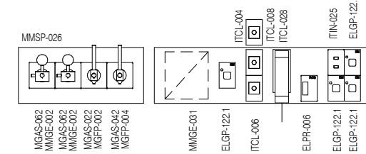
ELEVATION 4 (1 : 25 @ A3)
