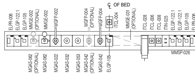
ELEVATION 5 (1 : 25 @ A3)
