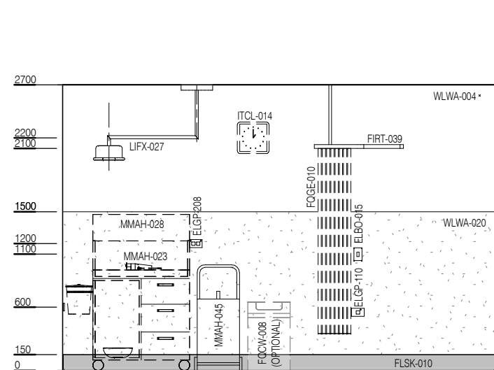
ELEVATION 5 (1 : 25 @ A3)
