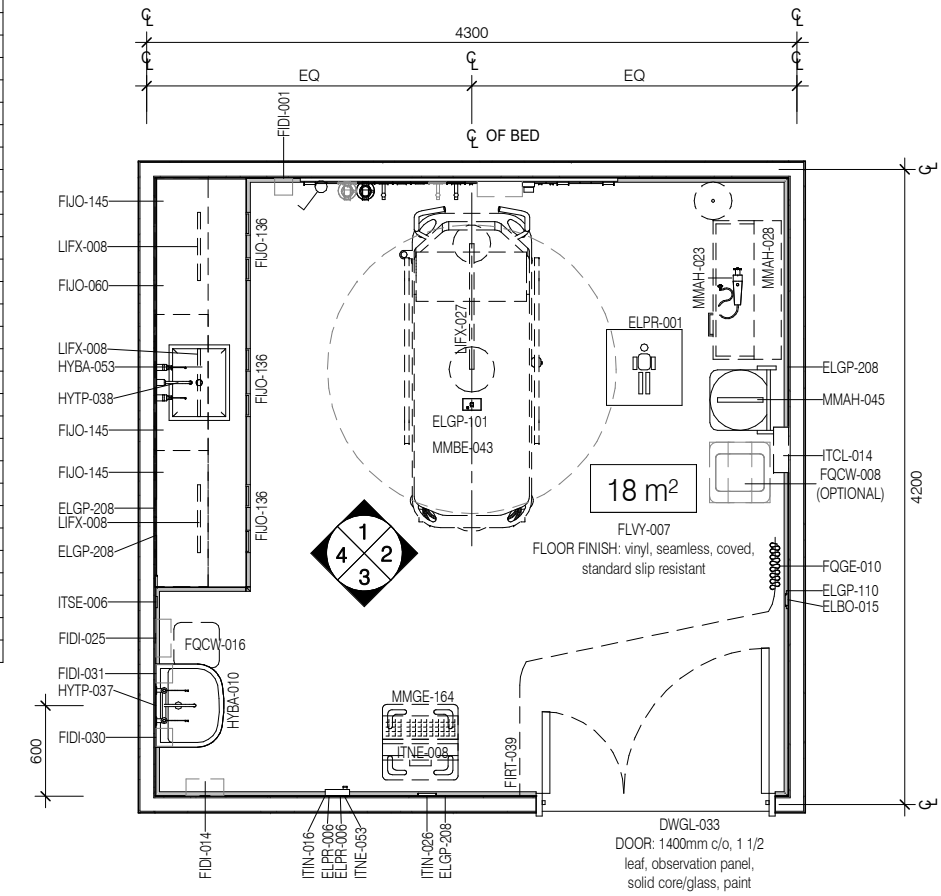
PLAN
