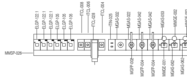
ELEVATION 5 ( 1 : 25 @ A3 )
