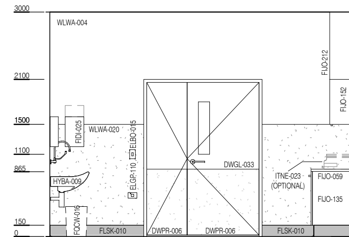
ELEVATION 5 (1 : 25 @ A3)
