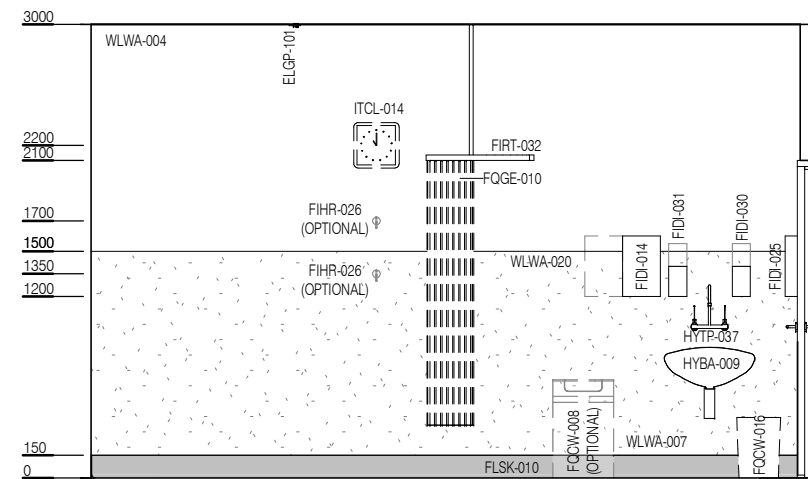
ELEVATION 5 (1 : 25 @ A3)
