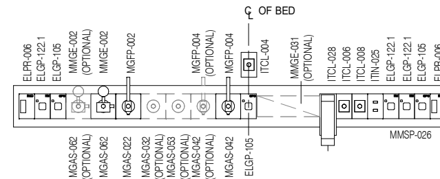
ELEVATION 5 (1 : 25 @ A3)
