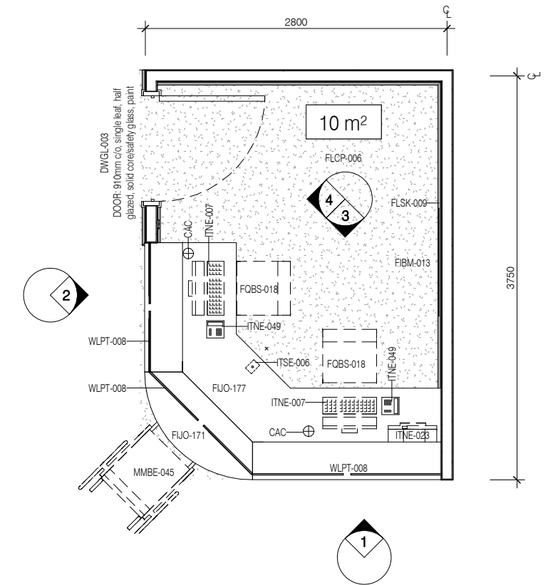
PLAN
