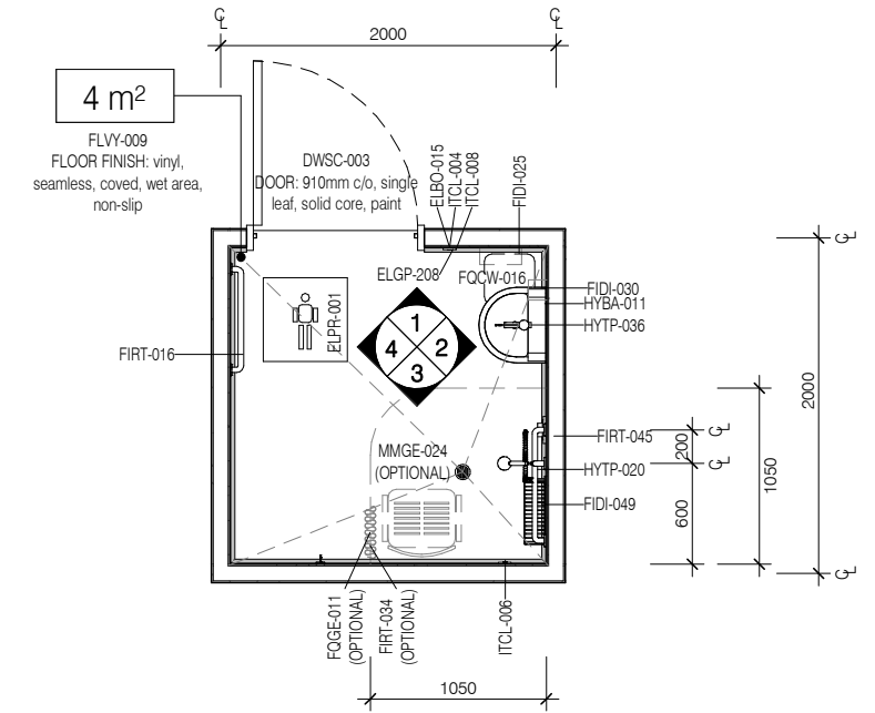
PLAN
