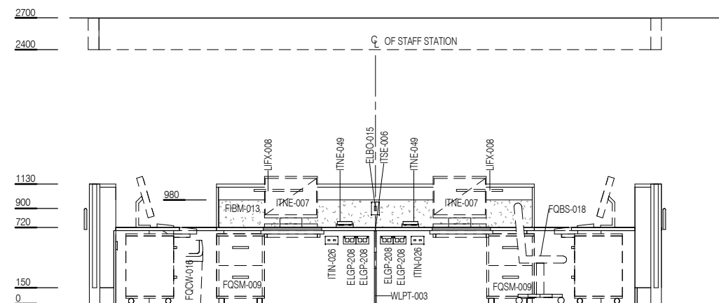
ELEVATION 5 ( 1 : 50 @ A3 )
