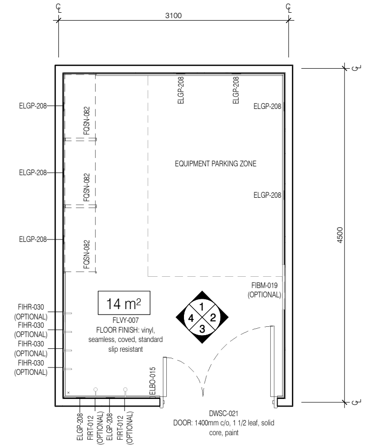
PLAN
