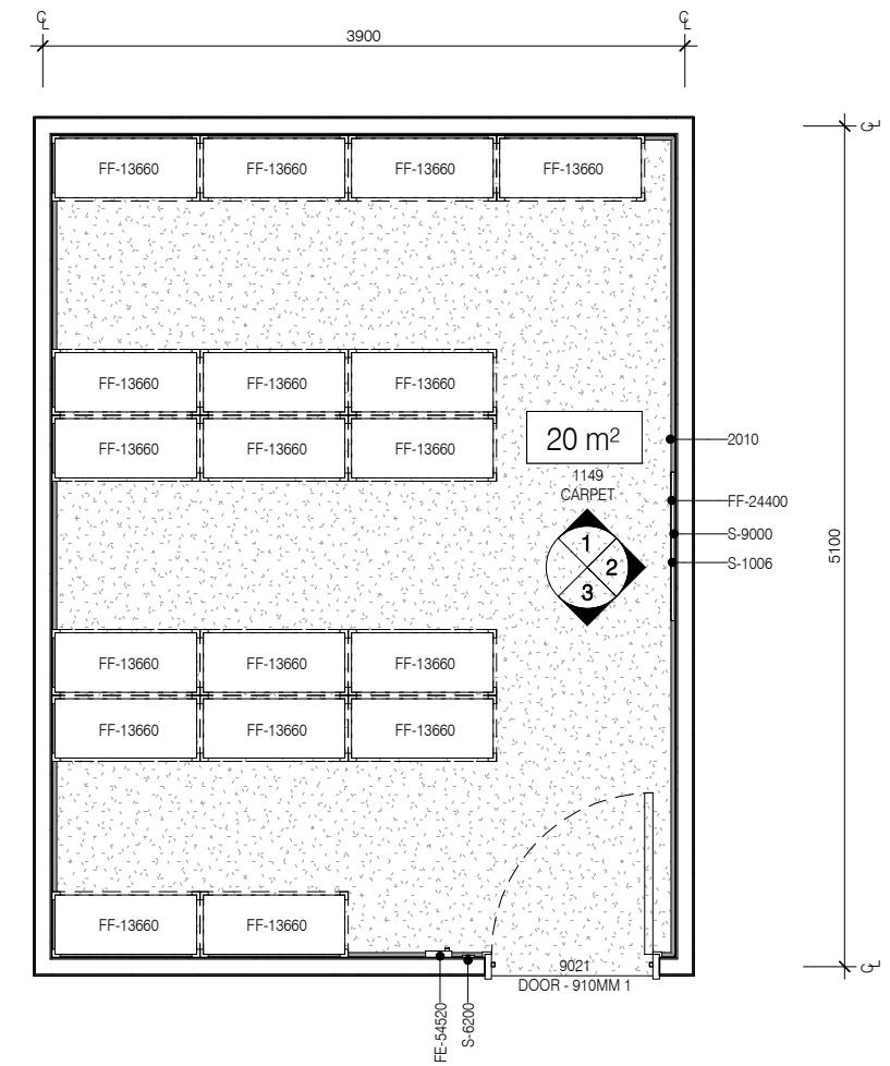
PLAN
