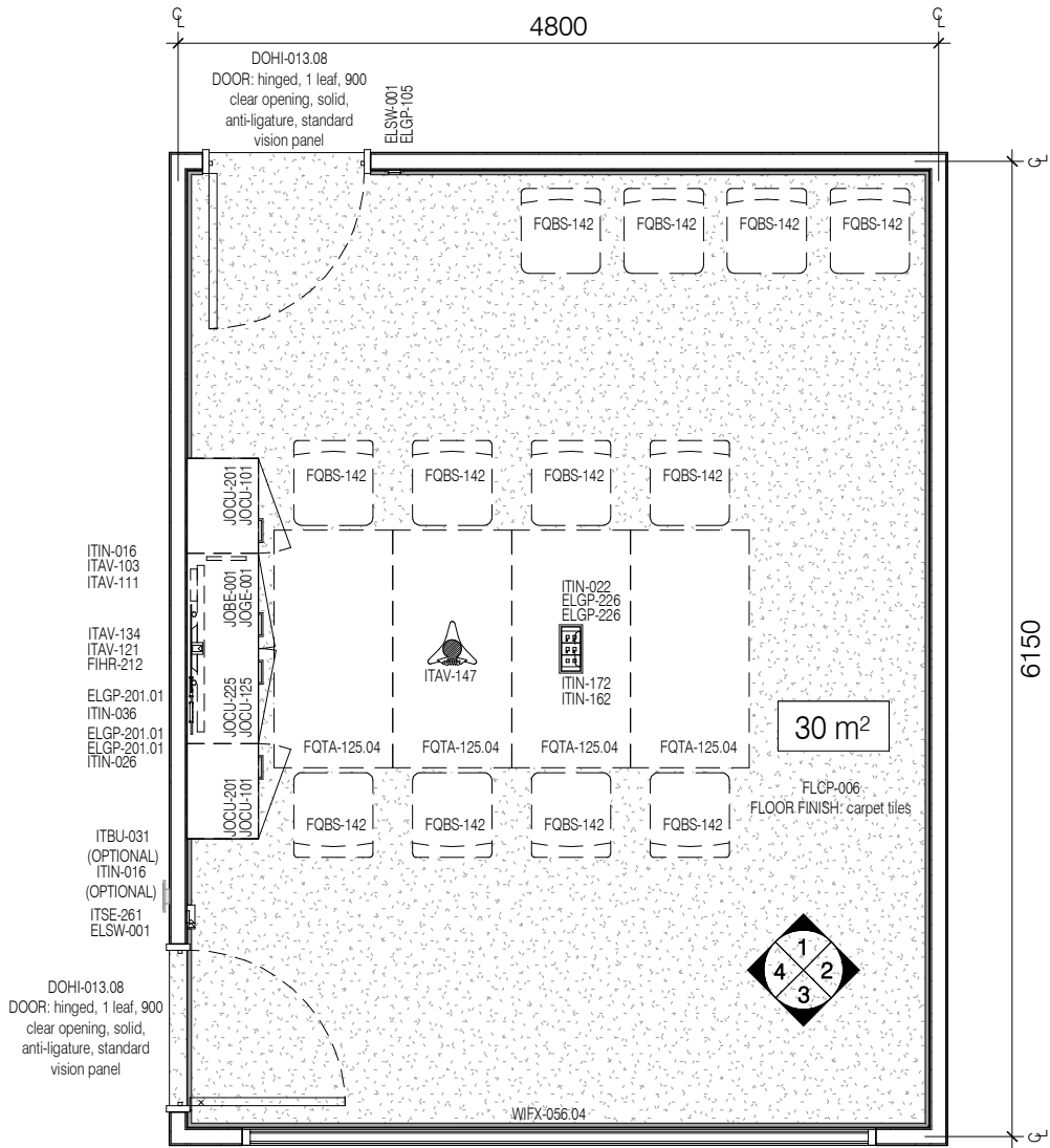
PLAN
