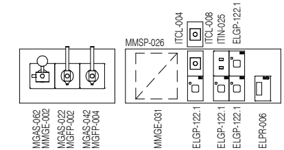
ELEVATION 5 ( 1 : 25 @ A3 )
