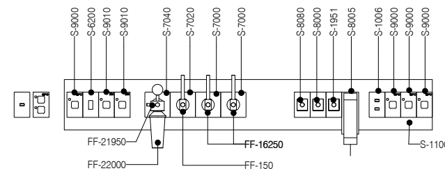
ELEVATION 5 ( 1 : 25 @ A3 )
