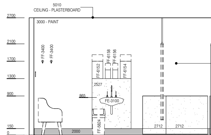
ELEVATION 5 ( 1 : 25 @ A3 )
