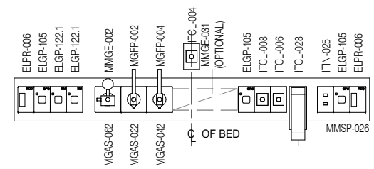
ELEVATION 5 ( 1 : 25 @ A3 )
