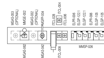
ELEVATION 5 ( 1 : 25 @ A3 )
