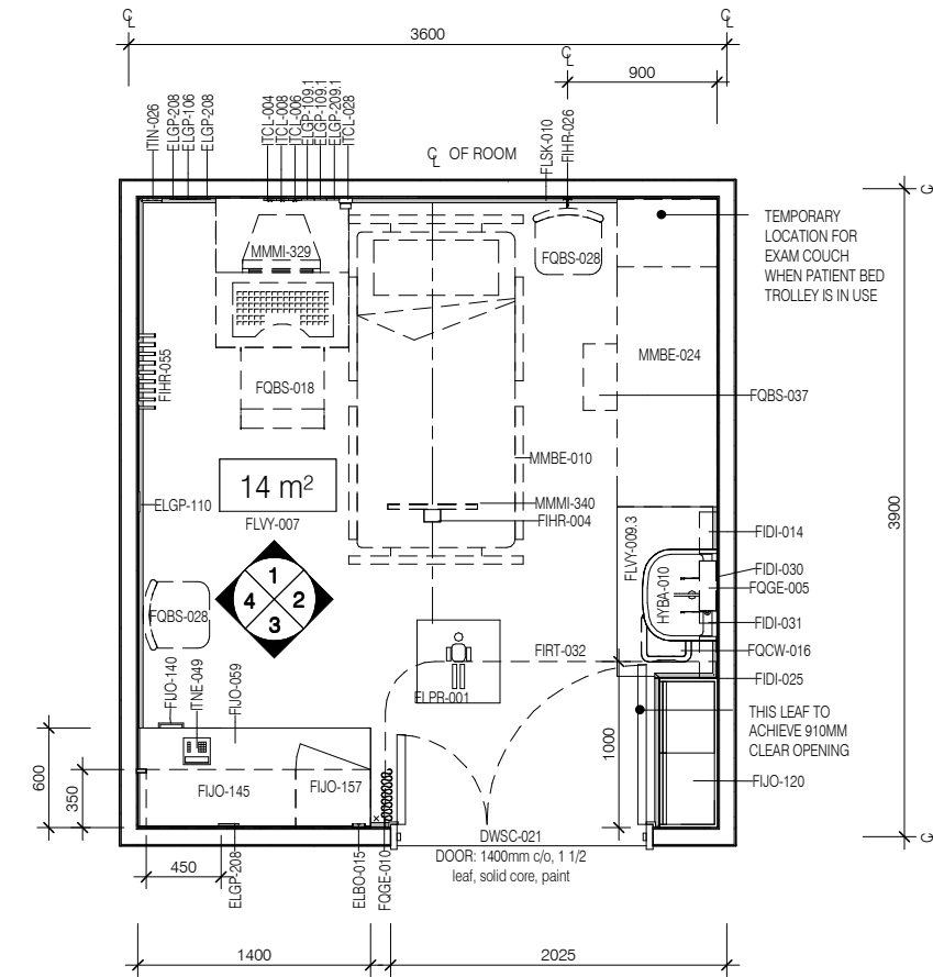
PLAN
