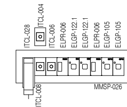
ELEVATION 5 ( 1 : 25 @ A3 )
